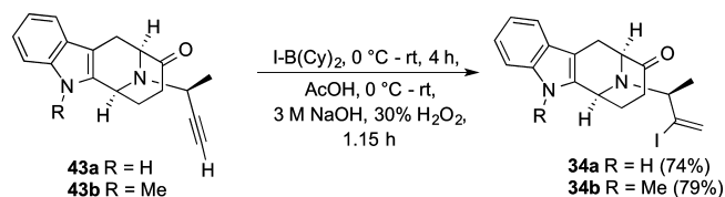
Scheme 7. Haloboration of the Acetylenic Tetracyclic Ketones 43a/b
